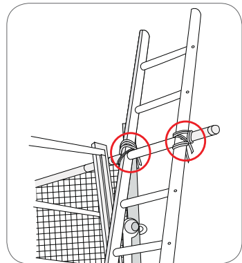
Figure 7: Provision for secured handhold landing point.
