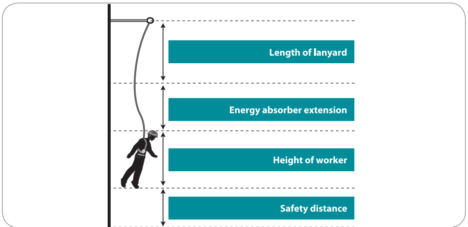
Figure 15: A graphical representation of the formula for calculating clearance height.
