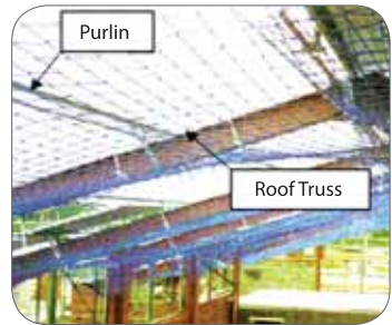
Figure 12: Safety nets in use for roof works.
